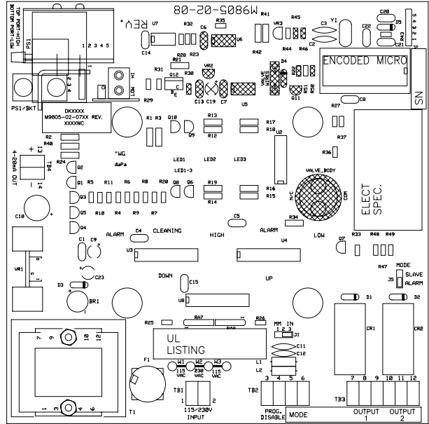
Airflow Controller Keypad and Printed Circuit Board
