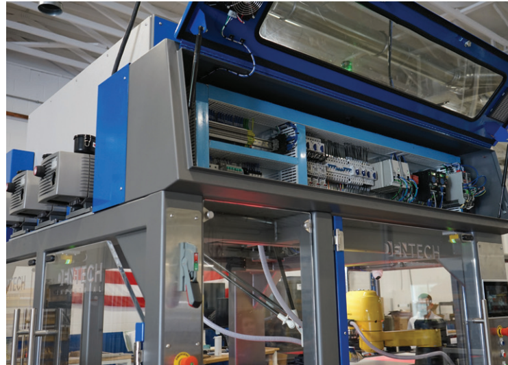
Electrical controls integrated into cell frame
